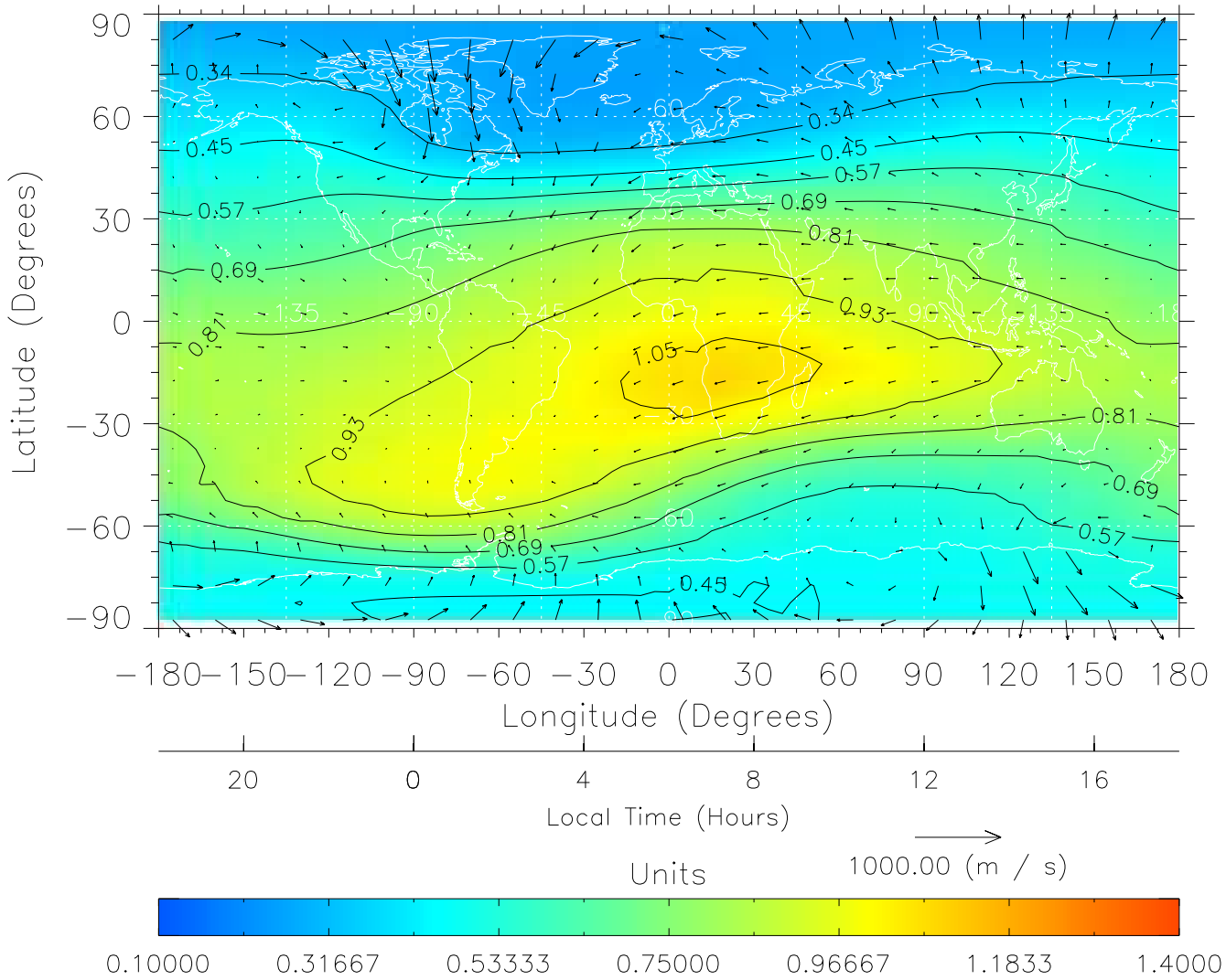
TIME-GCM MAP \Sigma O/N_2 with Neutral Wind vectors ZP = 2.00 UT = 6.00 DOY = 109
