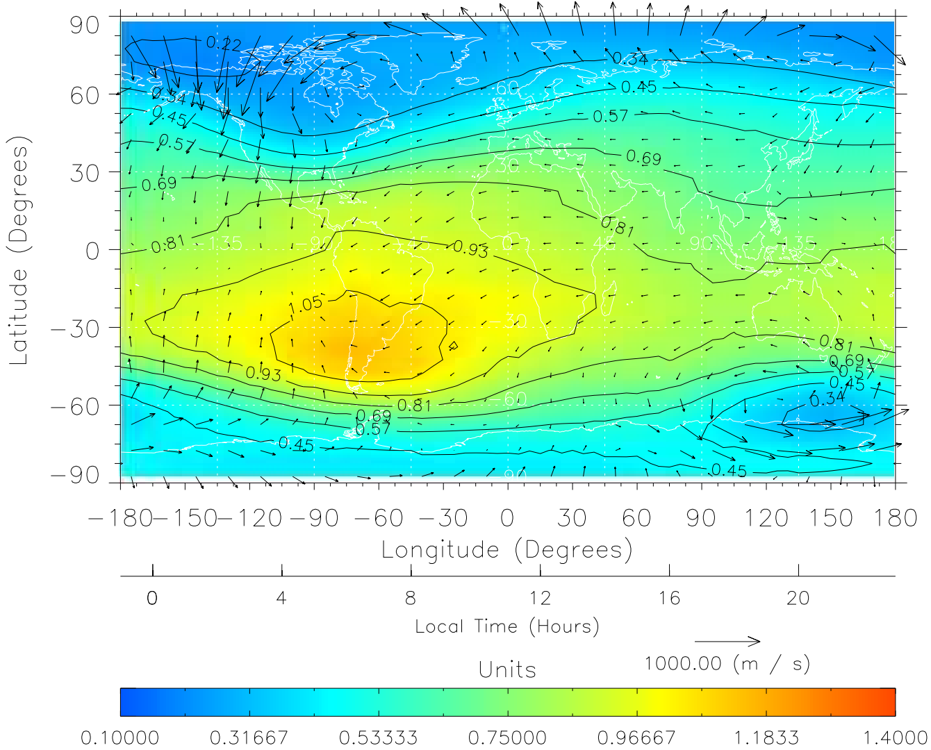
TIME-GCM MAP \Sigma O/N_2 with Neutral Wind vectors ZP = 2.00 UT = 11.00 DOY = 109
