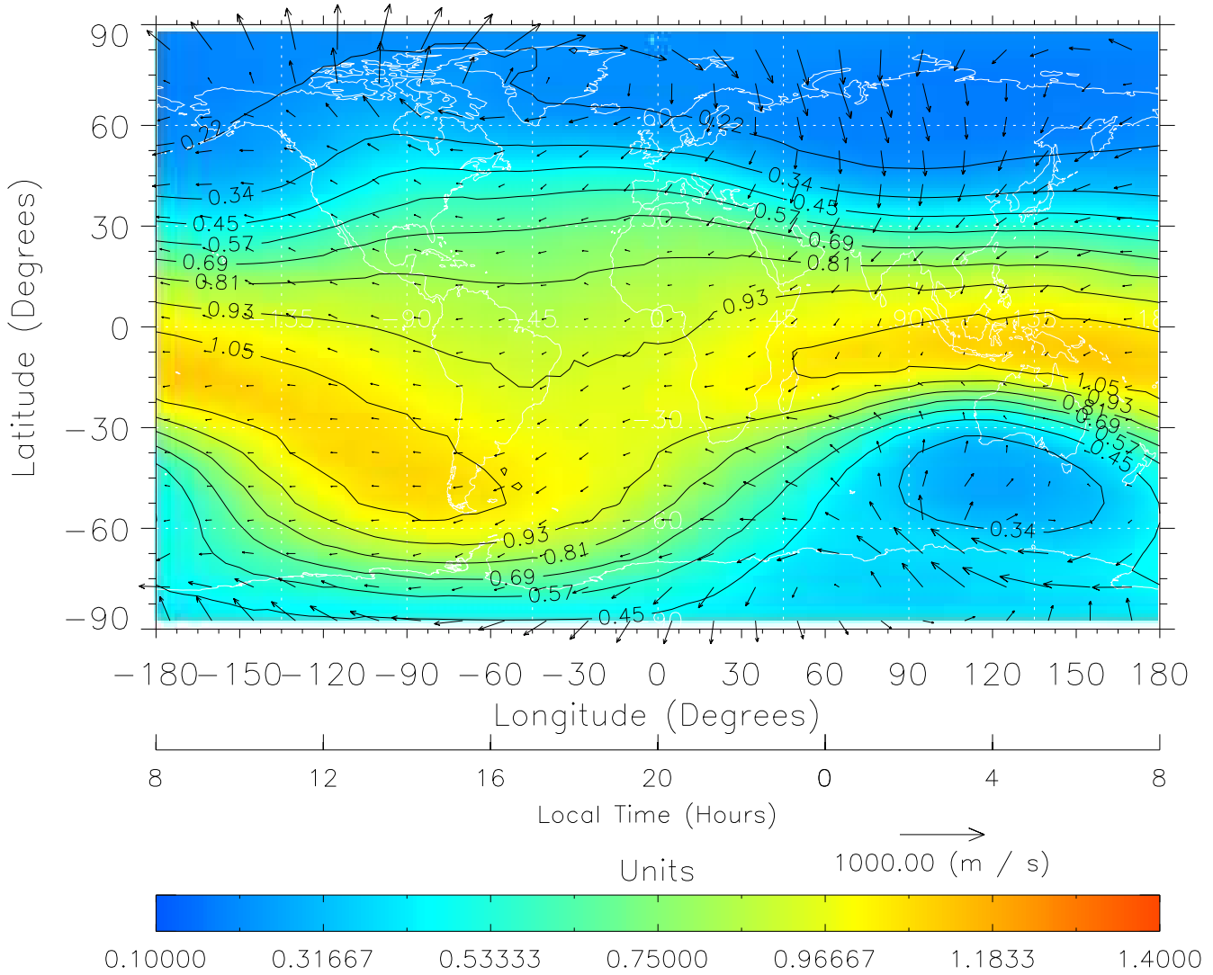
TIME-GCM MAP \Sigma O/N_2 with Neutral Wind vectors ZP = 2.00 UT = 20.00 DOY = 109
