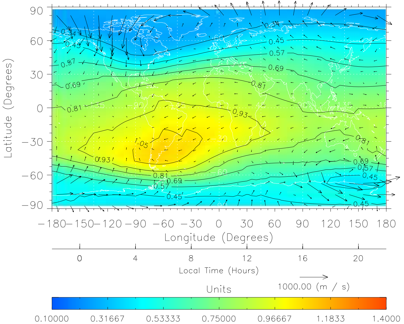
TIME-GCM MAP \Sigma O/N_2 with Neutral Wind vectors ZP = 2.00 UT = 10.00 DOY = 109
