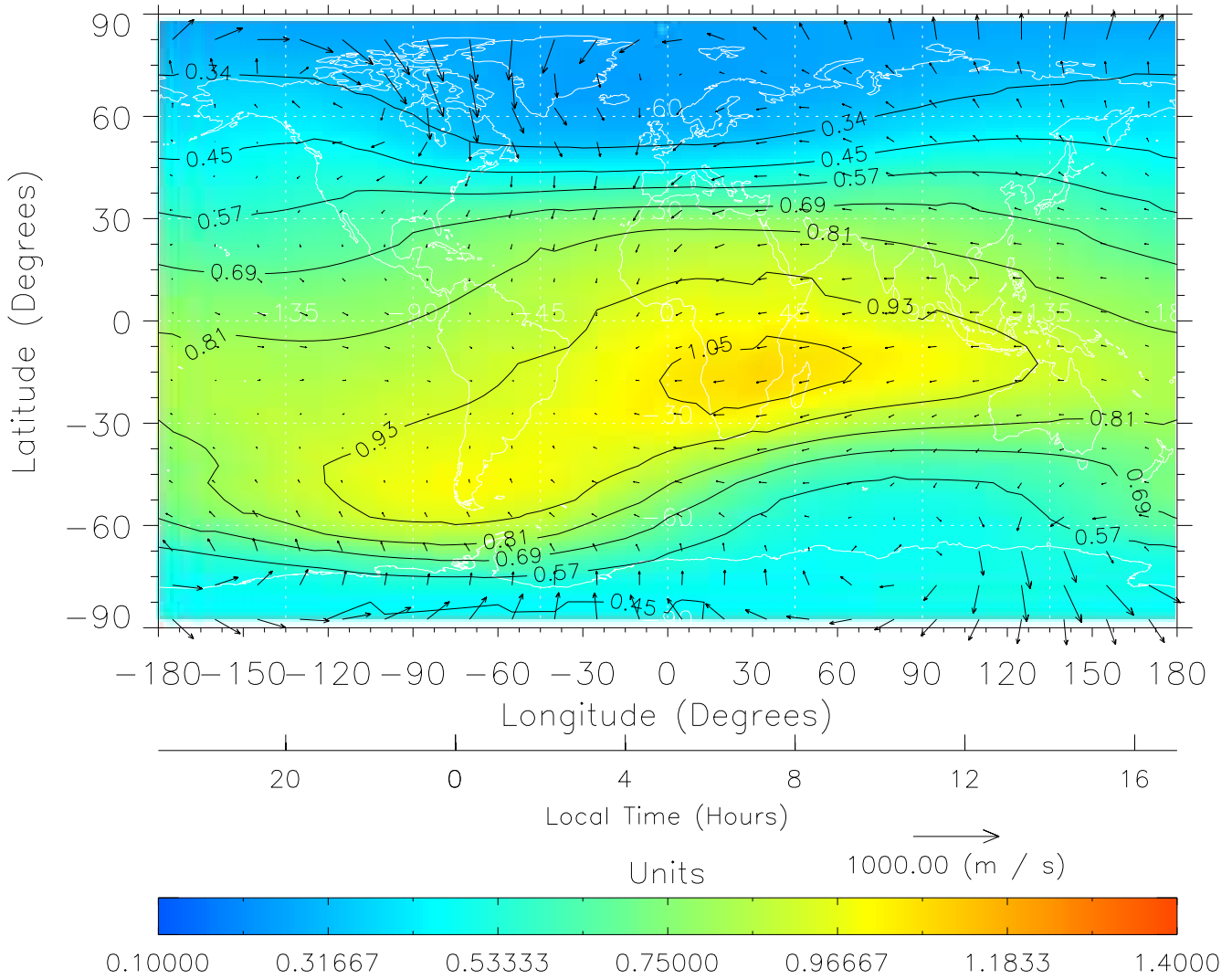
TIME-GCM MAP \Sigma O/N_2 with Neutral Wind vectors ZP = 2.00 UT = 5.00 DOY = 109
