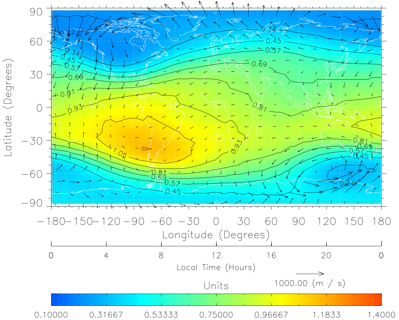
TIME-GCM MAP \Sigma O/N_2 with Neutral Wind vectors ZP = 2.00 UT = 12.00 DOY = 109
