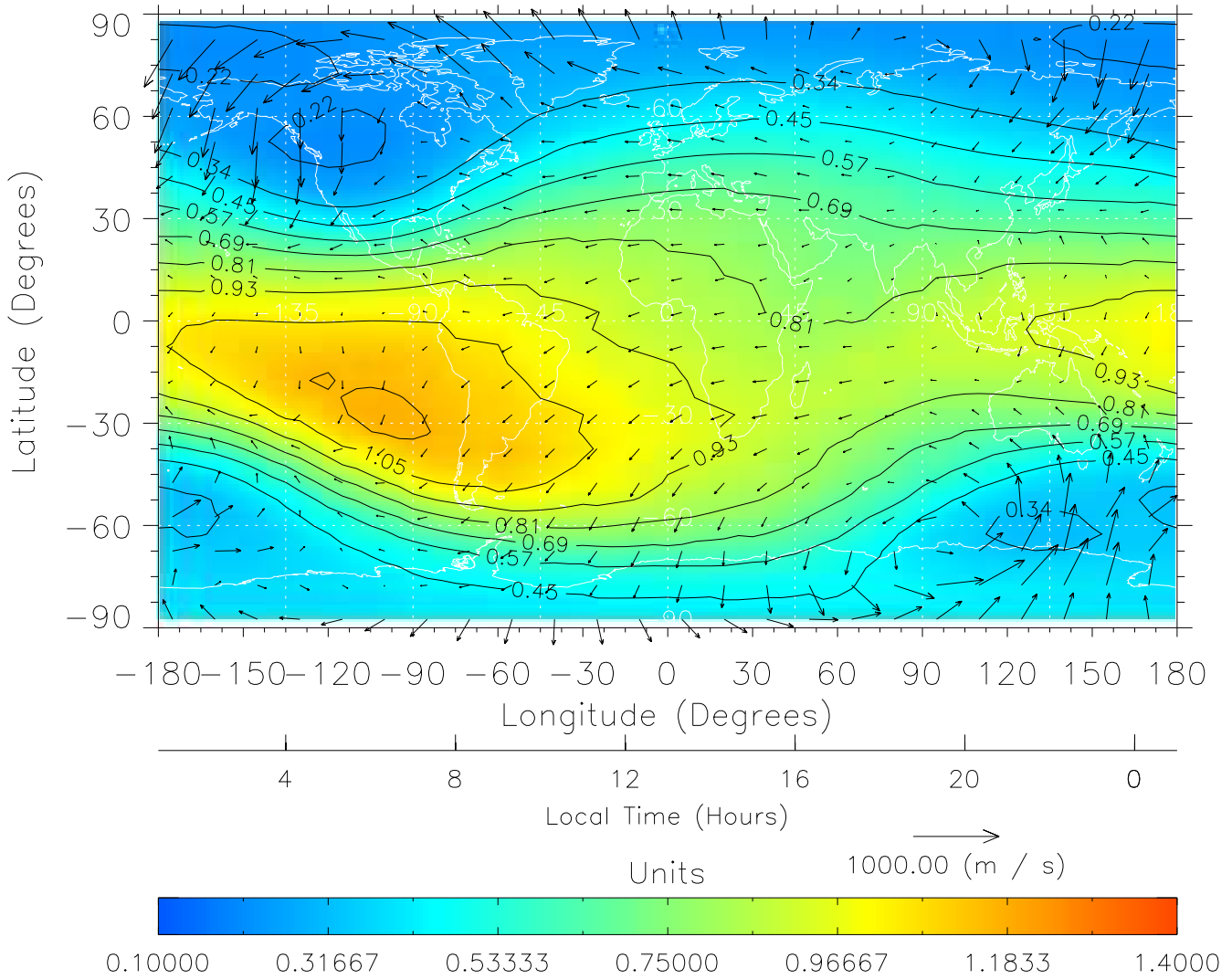
TIME-GCM MAP \Sigma O/N_2 with Neutral Wind vectors ZP = 2.00 UT = 13.00 DOY = 109
