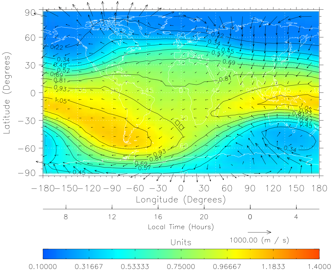
TIME-GCM MAP \Sigma O/N_2 with Neutral Wind vectors ZP = 2.00 UT = 18.00 DOY = 109
