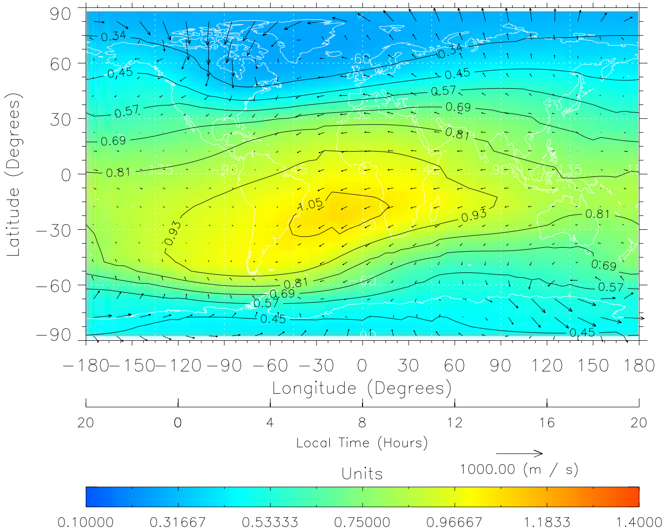
TIME-GCM MAP \Sigma O/N_2 with Neutral Wind vectors ZP = 2.00 UT = 8.00 DOY = 109
