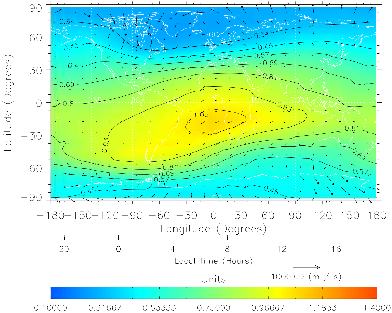
TIME-GCM MAP \Sigma O/N_2 with Neutral Wind vectors ZP = 2.00 UT = 7.00 DOY = 109
