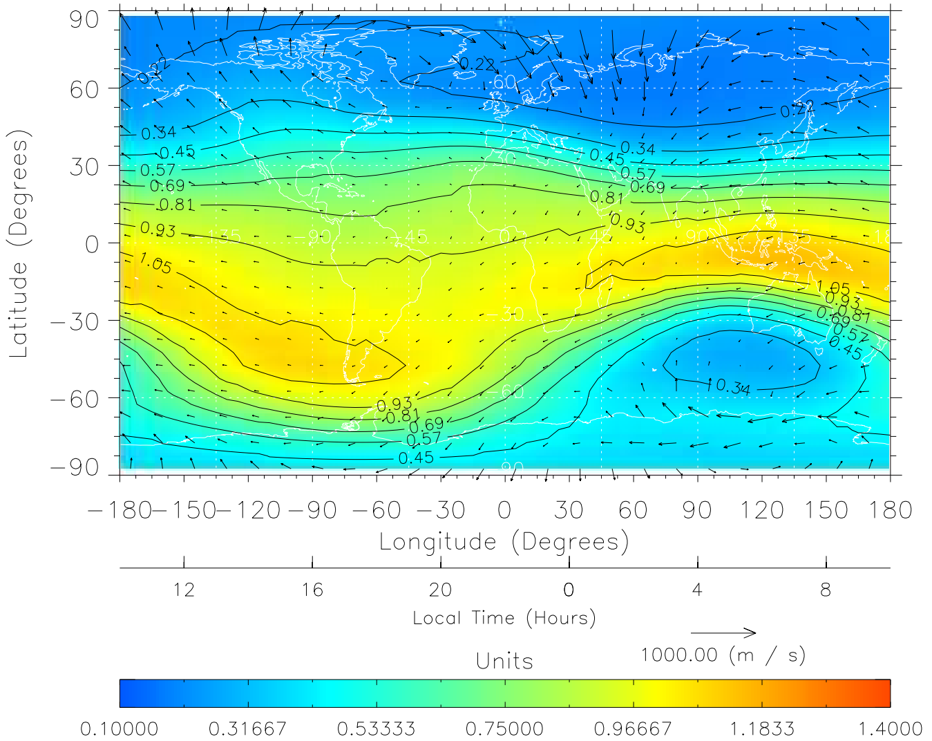
TIME-GCM MAP \Sigma O/N_2 with Neutral Wind vectors ZP = 2.00 UT = 22.00 DOY = 109
