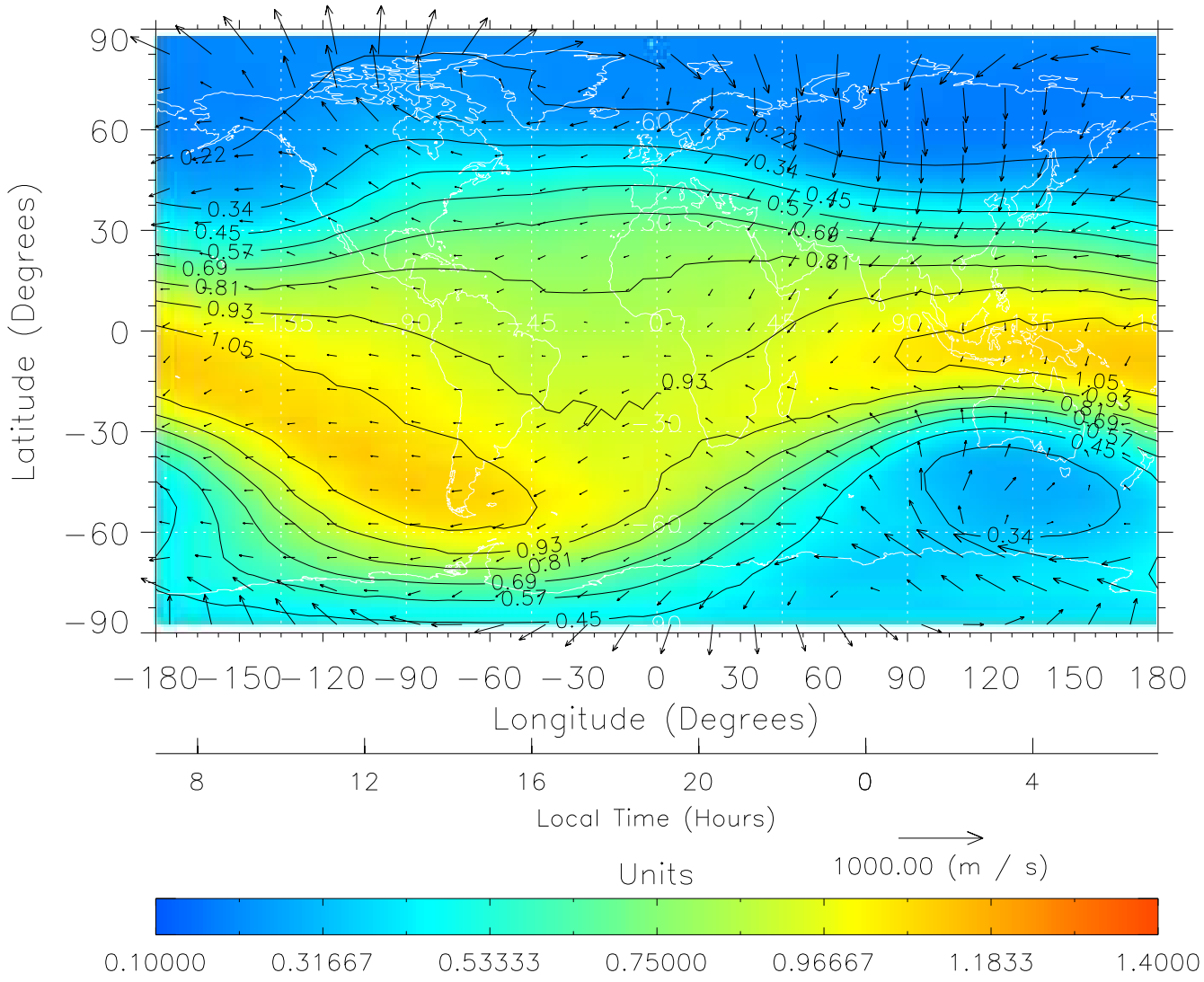
TIME-GCM MAP \Sigma O/N_2 with Neutral Wind vectors ZP = 2.00 UT = 19.00 DOY = 109
