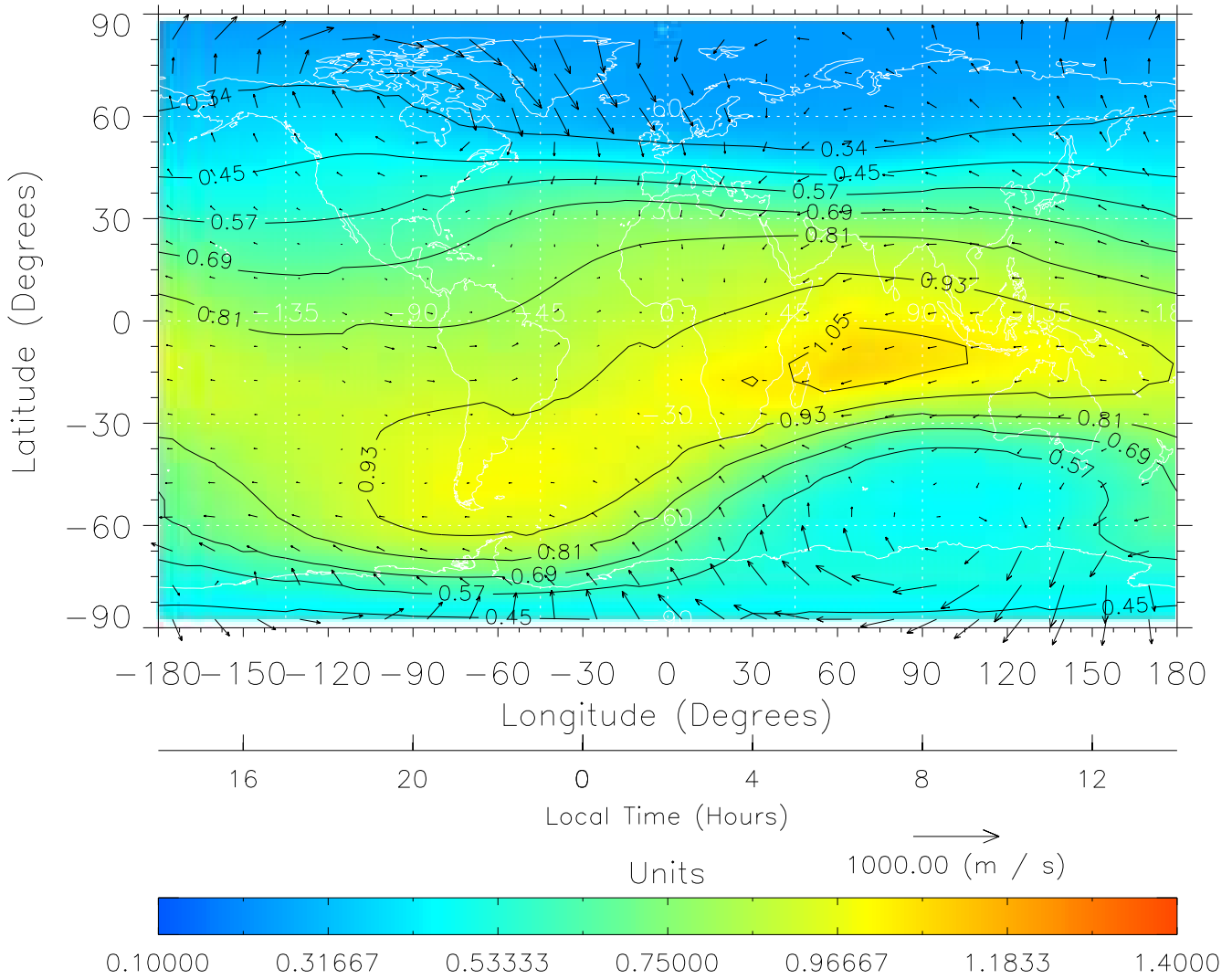
TIME-GCM MAP \Sigma O/N_2 with Neutral Wind vectors ZP = 2.00 UT = 2.00 DOY = 109
