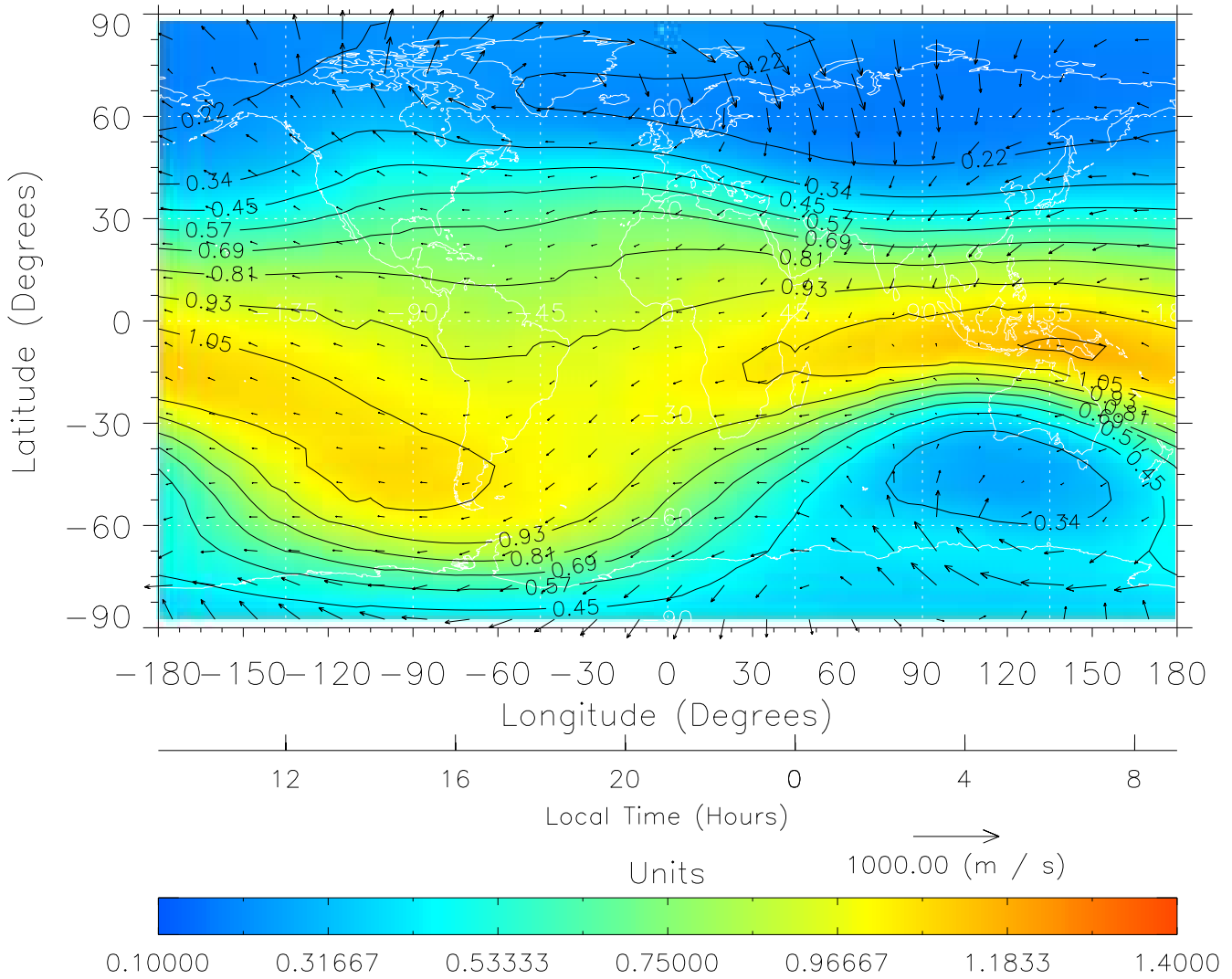
TIME-GCM MAP \Sigma O/N_2 with Neutral Wind vectors ZP = 2.00 UT = 21.00 DOY = 109
