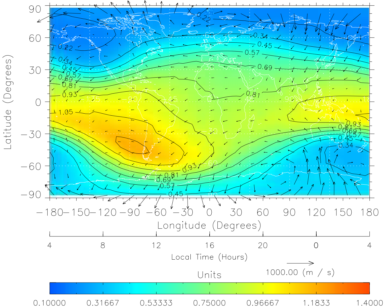
TIME-GCM MAP \Sigma O/N_2 with Neutral Wind vectors ZP = 2.00 UT = 16.00 DOY = 109
