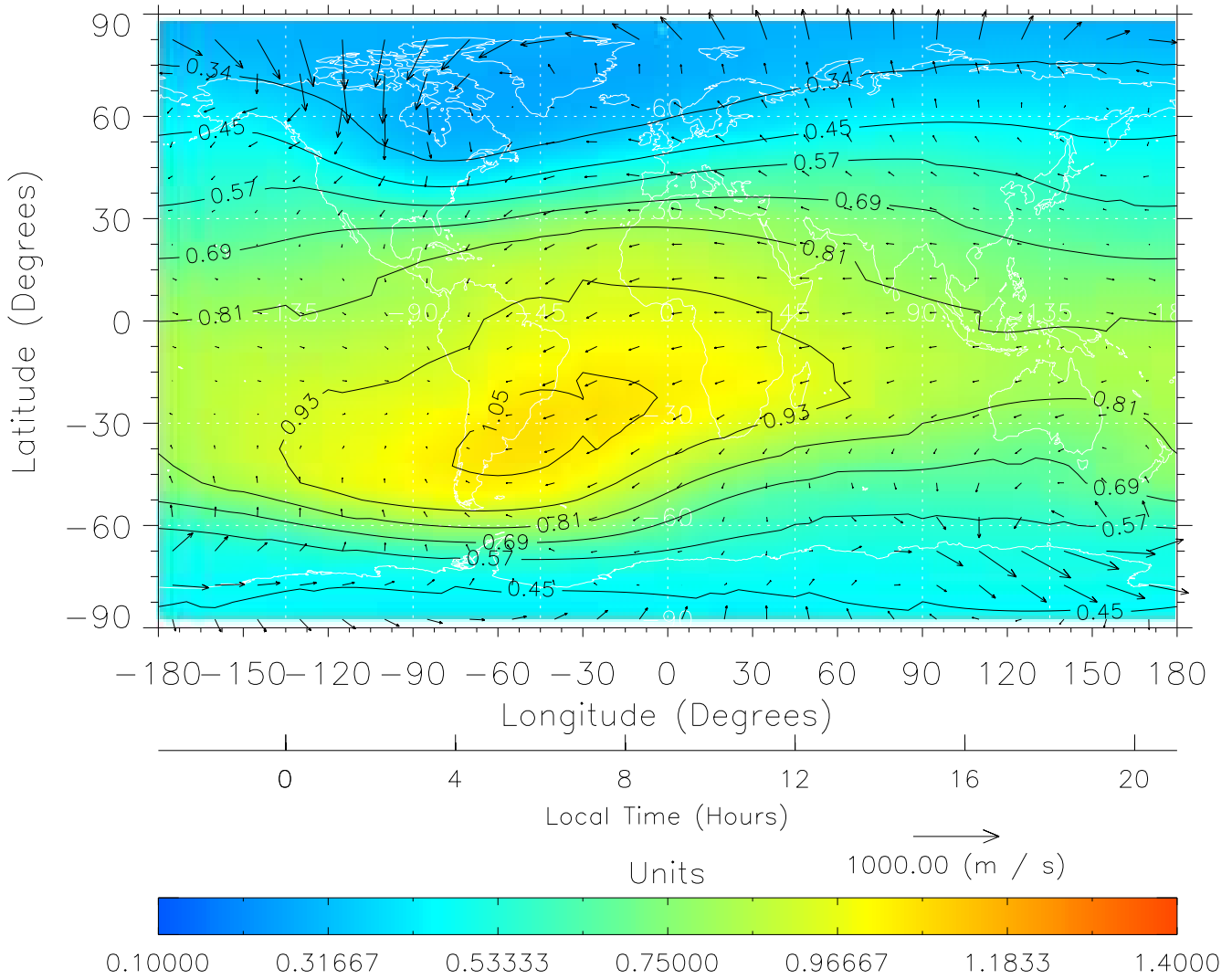
TIME-GCM MAP \Sigma O/N_2 with Neutral Wind vectors ZP = 2.00 UT = 9.00 DOY = 109
