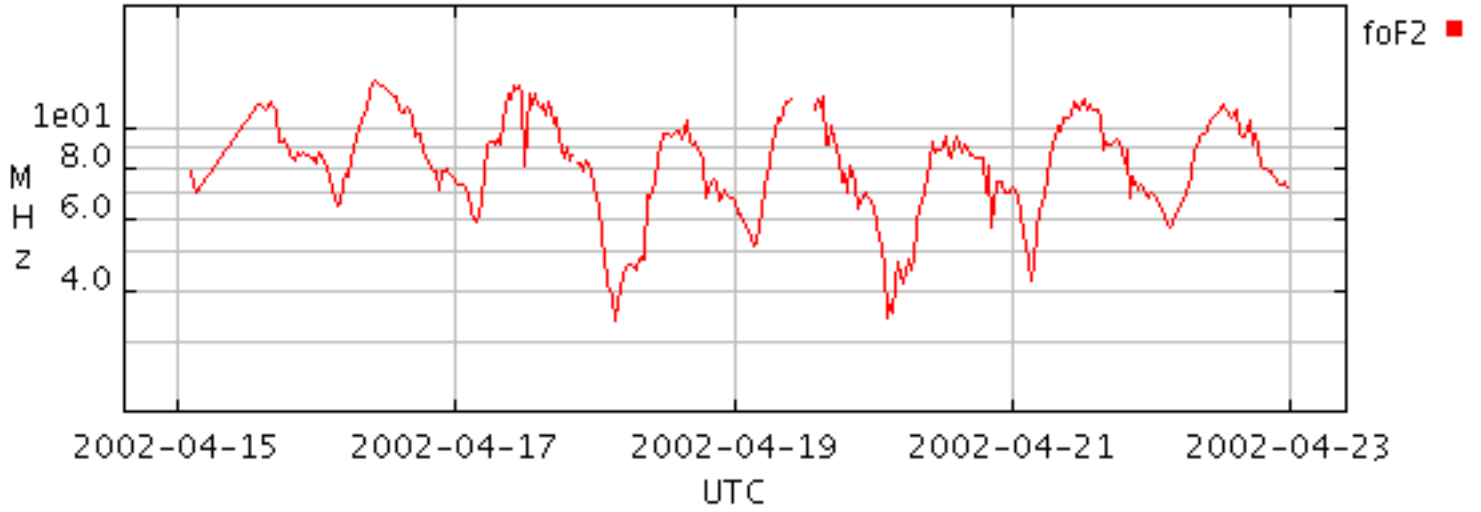
Layer frequencies@San Vito (undef sampling)
