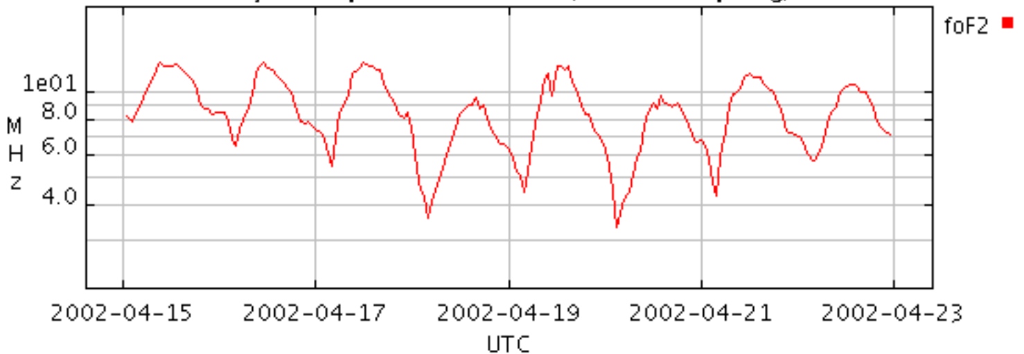
Layer frequencies@ROME (undef sampling)
