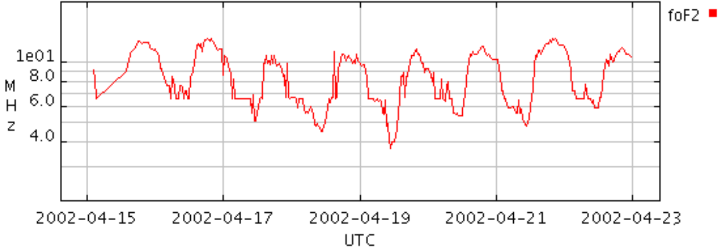
Layer frequencies@DYESS (undef sampling)
