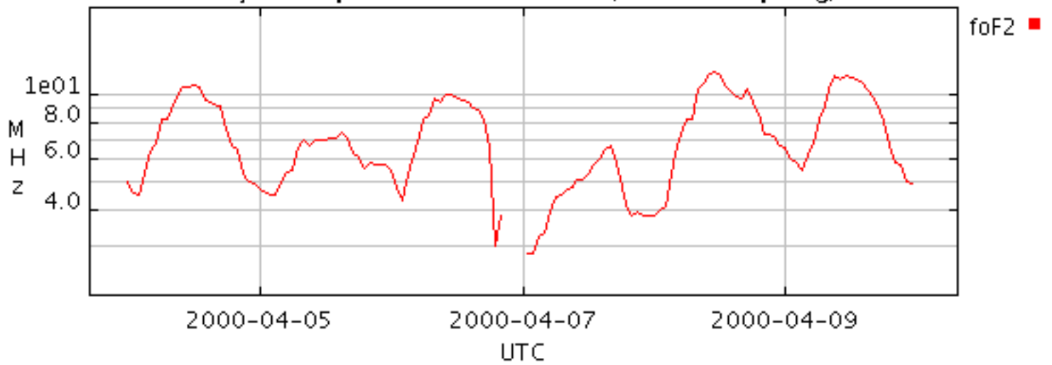
Layer frequencies@MOSCOW (undef sampling)
