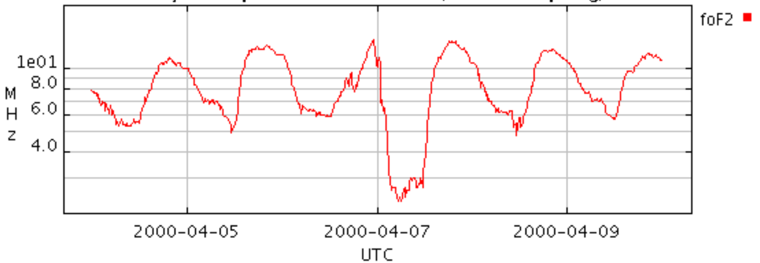
Layer frequencies@BOULDER (undef sampling)
