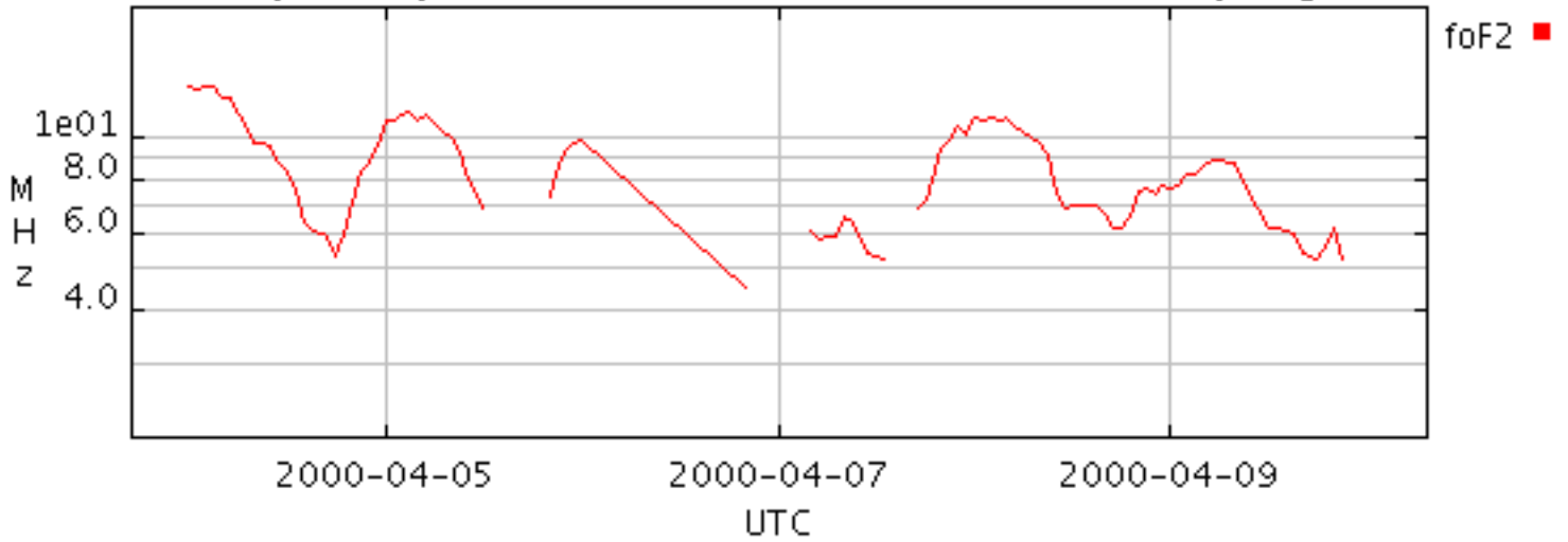
Layer frequencies@PETROPAVLOVSK (undef sampling)
