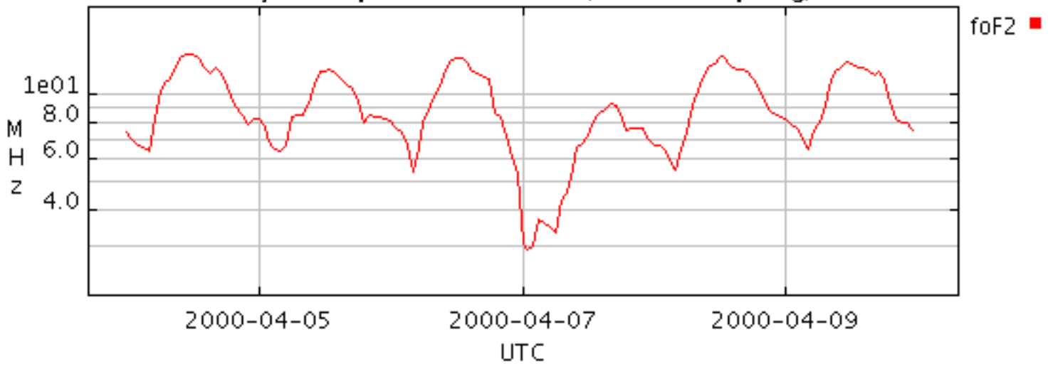
Layer frequencies@ROME (undef sampling)
