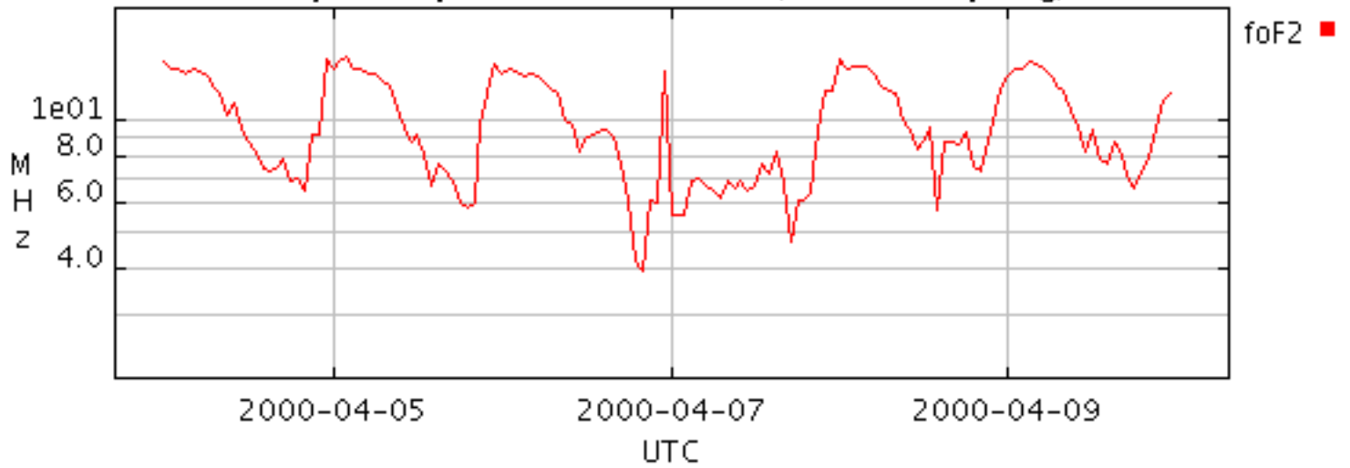
Layer frequencies@CAMDEN (undef sampling)
