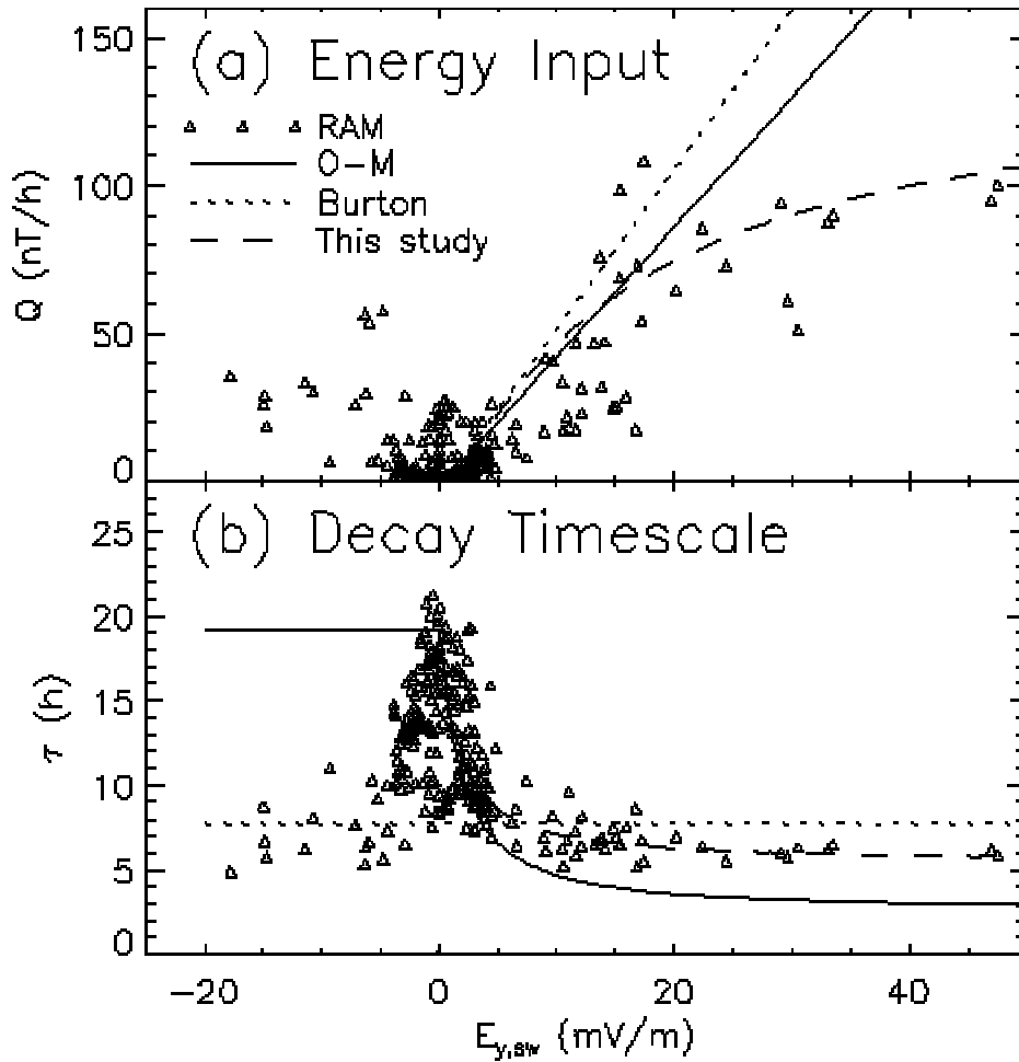
Figure 4. Plots of energy injection rates and decay times for the Bastille Day storm determined from the RAM algorithm, the original Burton equation, the O'Brien-McPherron equation, and the quadratic energy-conservation equation (this study).
