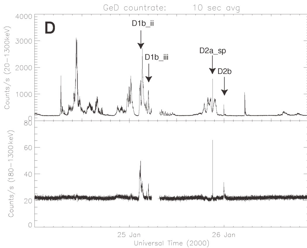
Figure 3.4: GeD count rate on Jan.24-26, 2000 in two energy channels: 20-1300 keV (top) and 180-1300 keV (bottom).
