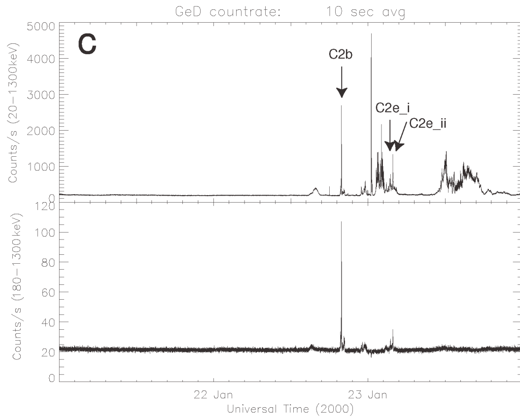
Figure 3.3: GeD count rate on Jan.21-23, 2000 in two energy channels: 20-1300 keV (top) and 180-1300 keV (bottom).
