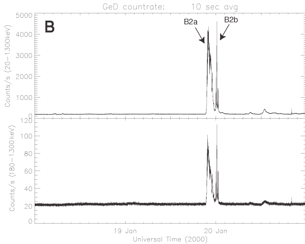
Figure 3.2: GeD count rate on Jan.18-20, 2000 in two energy channels: 20-1300 keV (top) and 180-1300 keV (bottom). MeV events are labeled and indicated by arrows.
