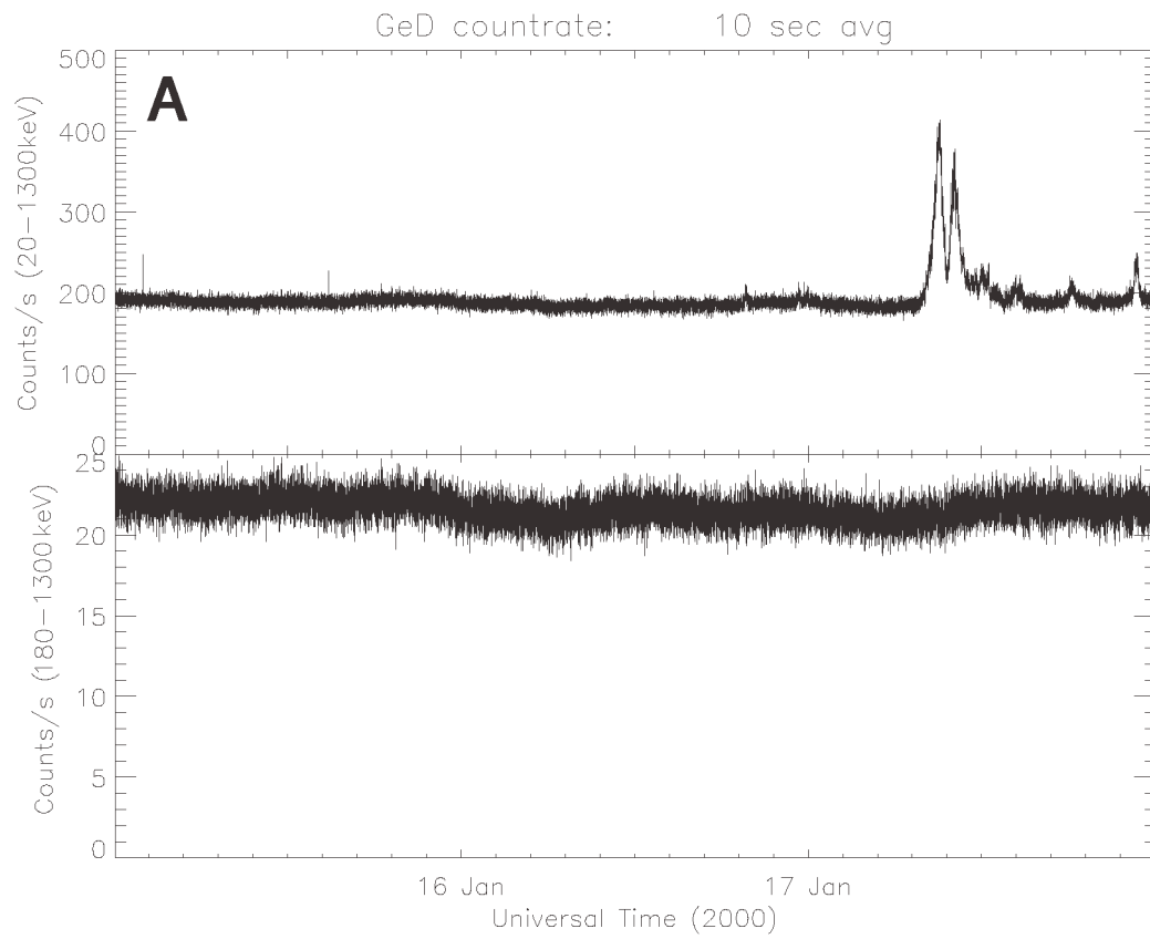
Figure 3.1: GeD count rate on Jan.15-17, 2000 in two energy channels: 20-1300 keV (top) and 180-1300 keV (bottom).
