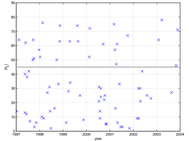
Fig. 6. Inclination angle \theta_C with respect to the ecliptic plane.
