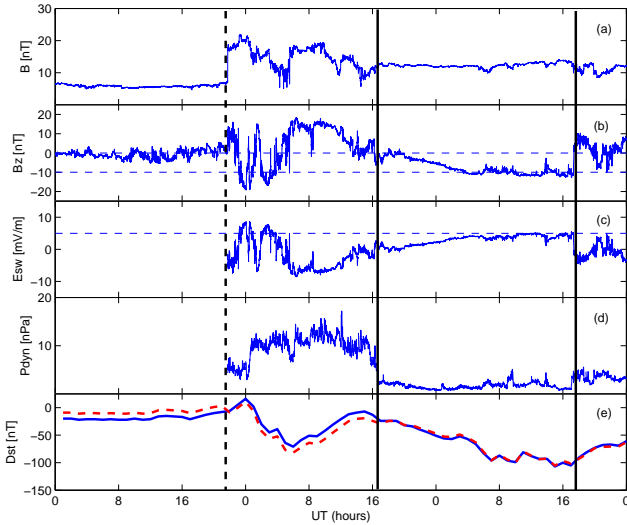
Fig. 13. Solar wind parameters and geomagnetic indices for a 3-day interval from 12–14 October 2000 measured by ACE. The figures from top to bottom are the same as in Fig. 9.
